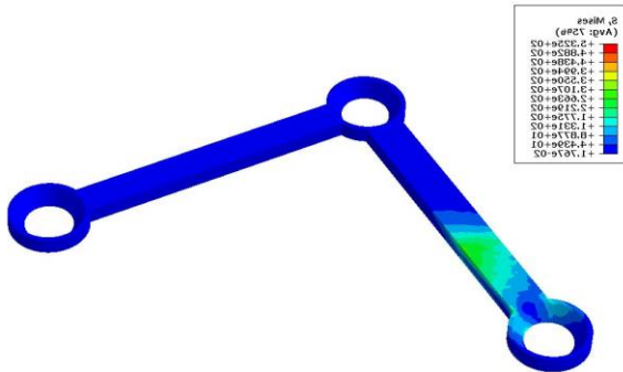
Fig. 2: (a) Miniplate
