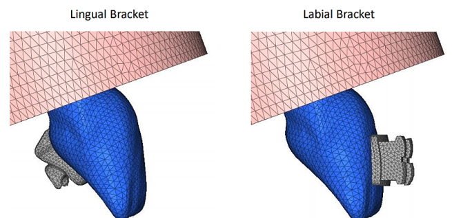
Fig. 4: Meshed models of maxillary central incisor with labial and lingual appliance systems.
