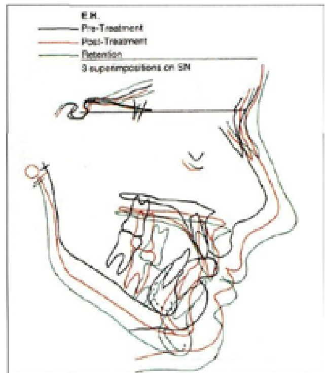
Fig. 2: Sella-Nasion Line
